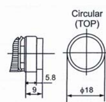
Ø18mm Form-3
