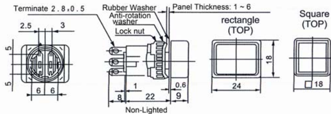
18x24mm Form-1
