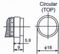
Ø18mm Form-3
