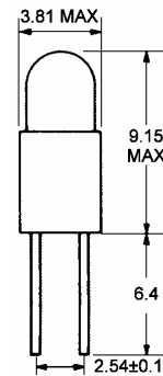
T-1 European Bi-pin (2.54) (Fig. D)
