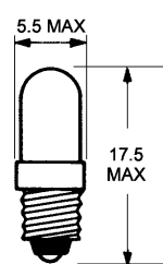
T-1 \frac{3}{4} Midget Screw (Fig. D)
