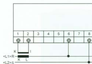
Single phase power factor meter
